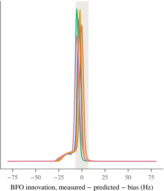
bto-bfo, 00:11 (shaded: \pm 7 Hz)
