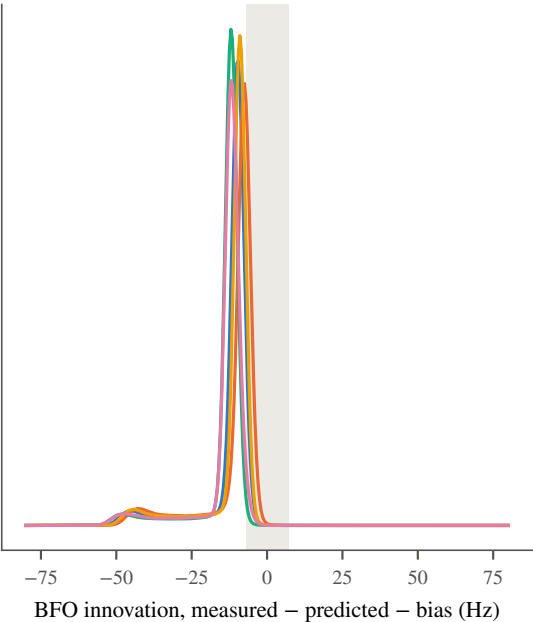
bto-bfo, 23:15 (shaded: \pm 7 Hz)
