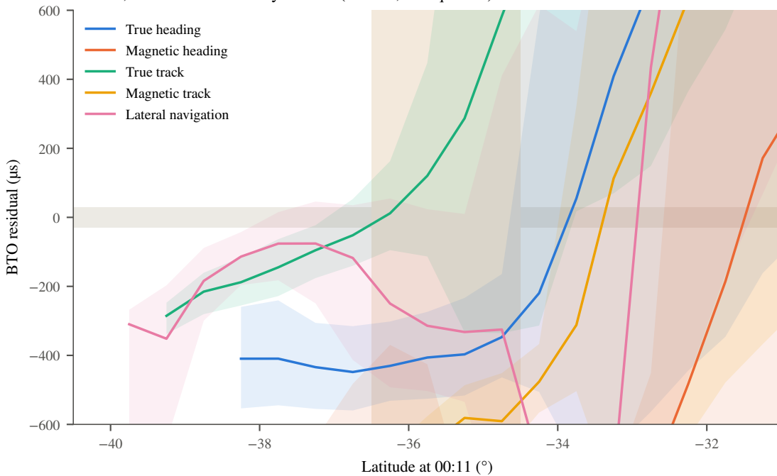
bto-only, 00:11: bto residual by latitude (median, interquartile)
