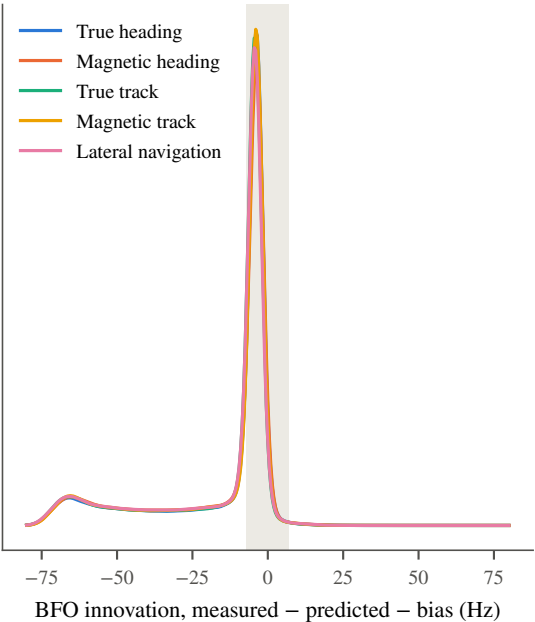
bto-bfo, 21:41 (shaded: \pm 7 Hz)
