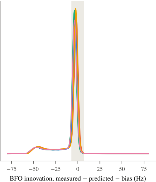
bto-bfo, 22:41 (shaded: \pm 7 Hz)
